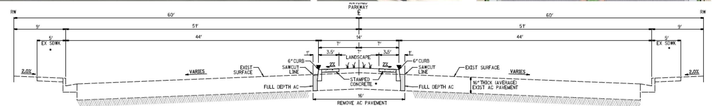
TYPICAL SECTION: ANTONIO PARKWAY
