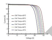
Current-Voltage Curve (LR4-60HPB-360M)
