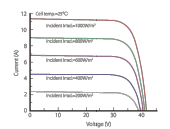
Current-Voltage Curve (LR4-60HPB-360M)
